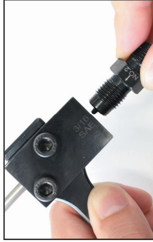
STEP 6: Remove the number 1 adapter and screw in the number 2 adapter and tighten with wrench.
