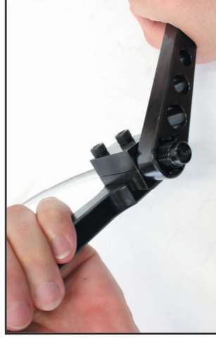
STEP 5: Remove the STOP adapter and screw in the number 1 adapter and tighten with wrench.
