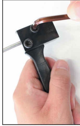
STEP 8: Remove the number 3 adapter and loosen the 2 x 5mm SHCS and remove hardline with double flare!
